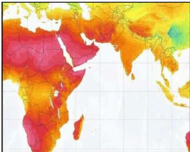
Fig. 4. Solar radiation map(Gulf-India)
