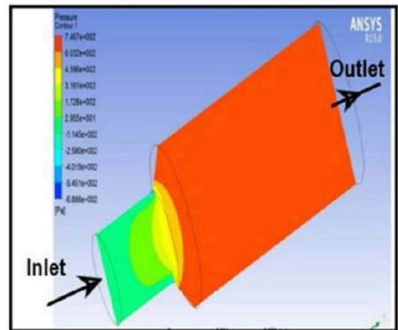
Fig. 6. Pressure contours of the nozzle
