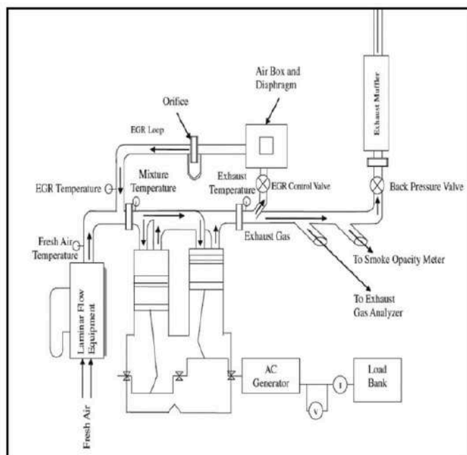
Fig.6. Exhaust Gas Recirculation
