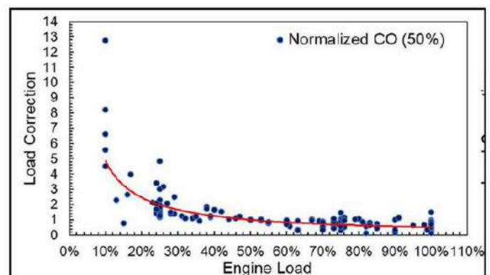
Fig. 14. Load Correction by Carbon Monoxide
