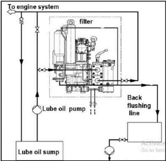
Fig. 2. Lubrication system line
