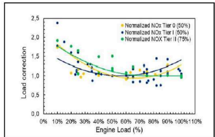
Fig. 12 Load Correction by Nitrogen Oxide
