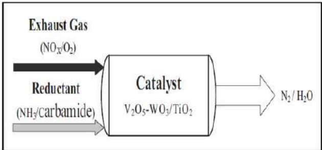
Fig.2. Process
