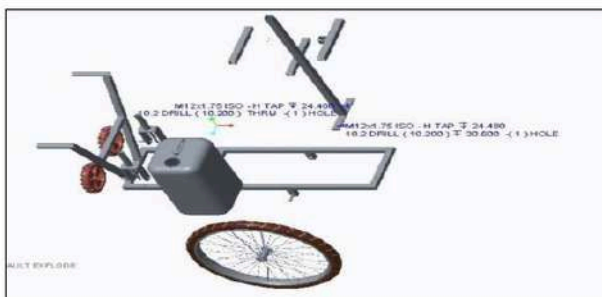
Fig.4. Exploded View
