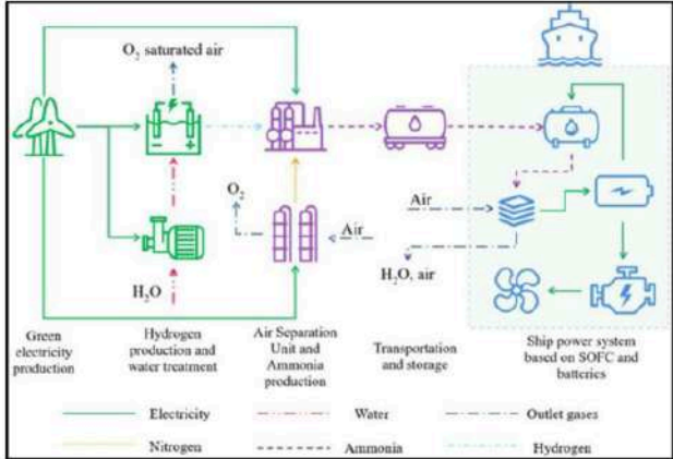
Fig. 2 Chart of processes of NH 3 production and usage in a ship with energy fully provided by renewable sources.
