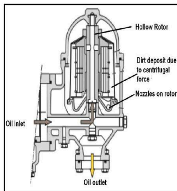
Fig. 1. Centrifugal automatic filter
