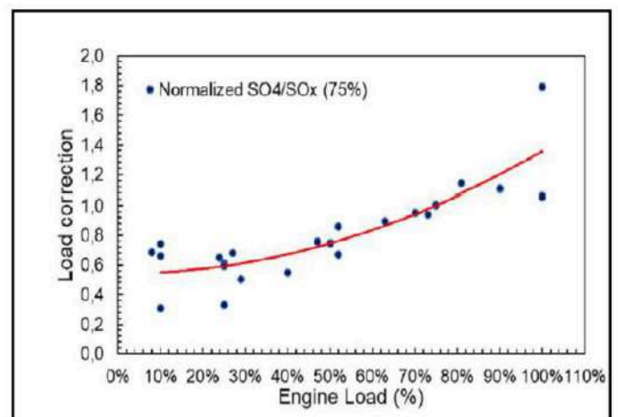
Fig. 13. Load Correction by Sulphur Oxide
