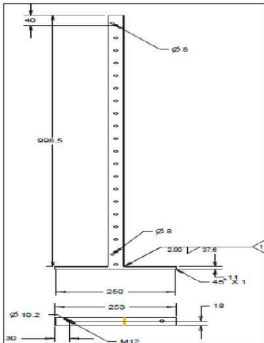
Fig. 2 Nozzle Strip
