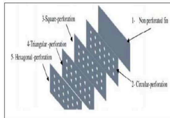
Fig. 3. Plate fins with different shape of perforation. [3]
