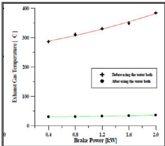
Fig. 11. Exhaust Gas Temperature
