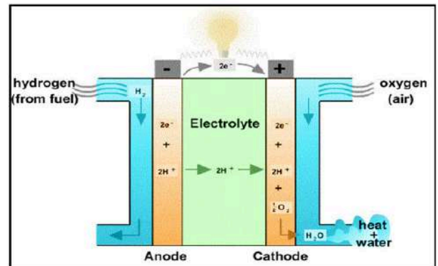
Fig. 5. Hydrogen Fuel Cell [15].
