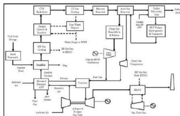
Fig. 1. IGCC Block Flow Diagram (Picture Credits : National Energy Technology Laboratory)
